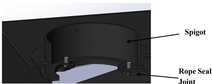
Fig. 1. Flue & Spigot Fitting
