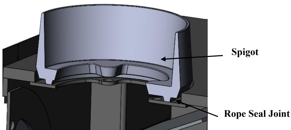
Fig. 1.Flue & Spigot Fitting
